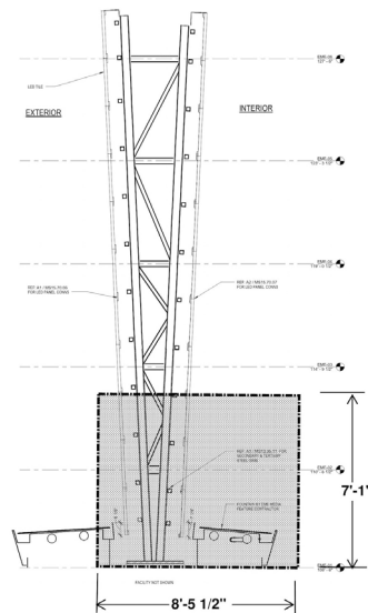
DIAGRAM 1B: F-1 Moment Vault Section
